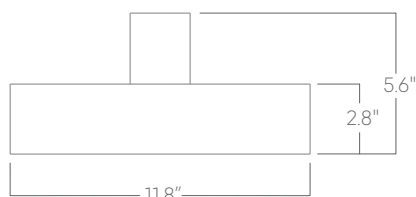
Saturn
