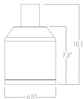
Mercury
