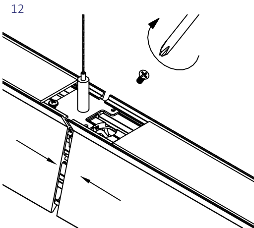
12 Use the provided 1/4-20 flat head screw to secure the connecting brackets. As you screw it in, the fixture will securely connect together. Tighten the connecting bracket screws again if needed.
