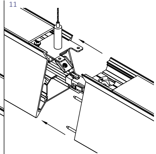
11 Align the two fixtures using the alignment pins and brackets. Warning: Keep hands clear of connection.
