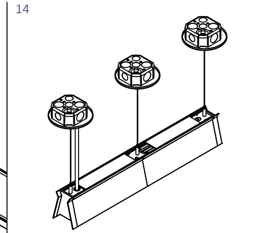
14 Fixture must be hung level at the desired height. If fixture is not level, light leaks may occur at the seam.
