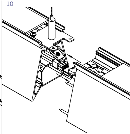
10 Before connecting the two fixtures, connect the wiring harness.
