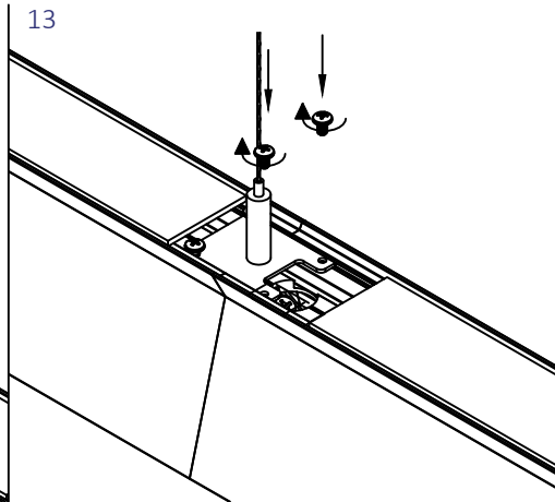
13 Use appropriate hardware to secure the middle suspension bracket in place. Reinstall the top lens as well if necessary.
