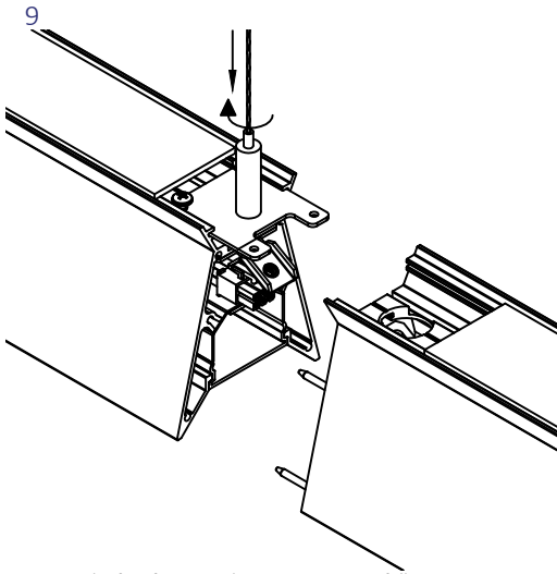
9 Mount the first fixture in the continuous run, following steps 1-8. Slide back the middle support bracket and screw on the cable gripper. If you have an UP/DN fixture, you may have to remove the top lens as well to perform the next steps.
