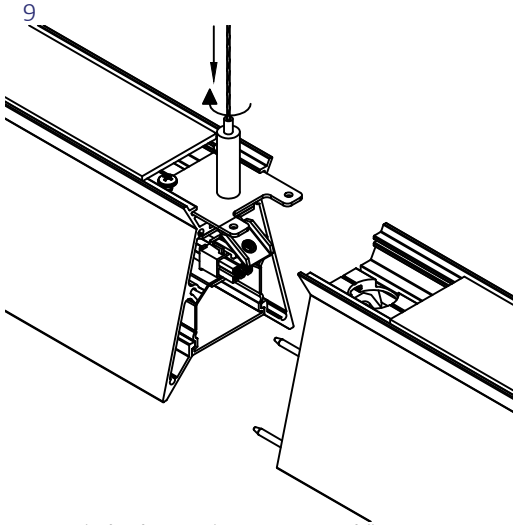
9 Mount the first fixture in the continuous run, following steps 1-8. Slide back the middle support bracket and screw on the cable gripper. If you have an UP/DN fixture, you may have to remove the top lens as well to perform the next steps.
