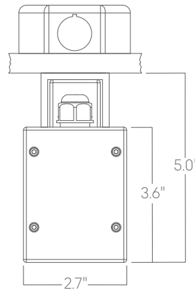
Surface mount
