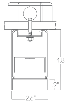
Surface mount
