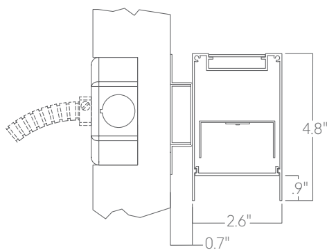
Wall mount
