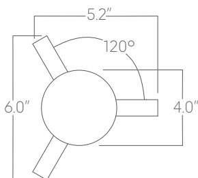
Three-Way 120° Connector
