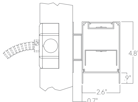
Wall mount
