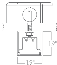
Surface mount
