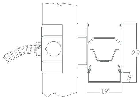
Wall mount
