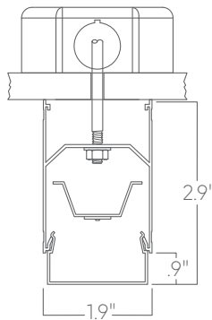
Surface mount
