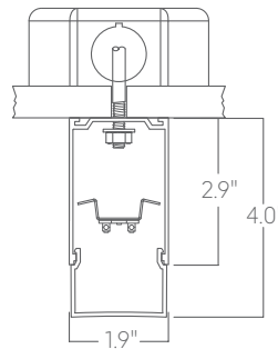
Surface mount Hard Ceiling
