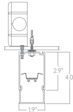
Surface mount T Bar clip
