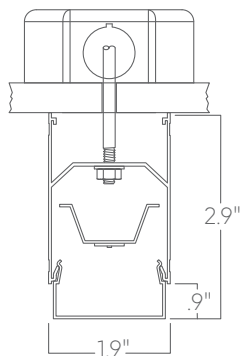
Surface mount
