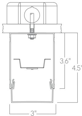
Surface mount
