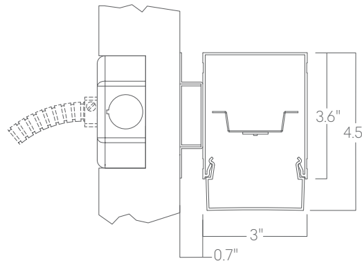
Wall mount
