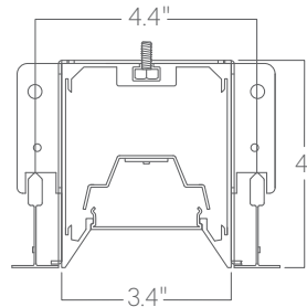
T15 15/16" tee grid
