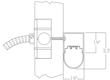
Wall mount
