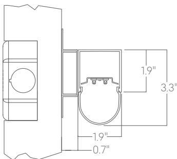
Wall mount
