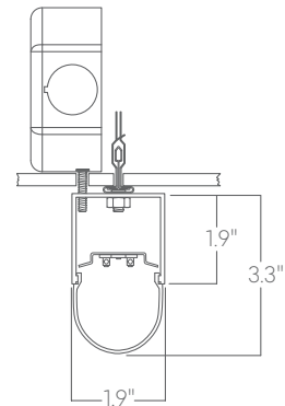
Surface mount T Bar clip
