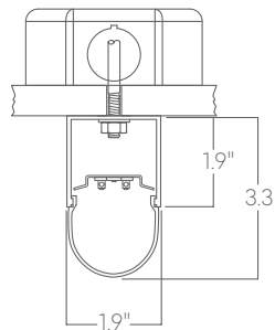
Surface mount Hard Ceiling
