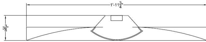
CROSS SECTION
