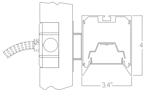
Wall mount
