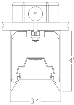
Surface mount
