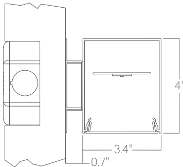
Wall mount
