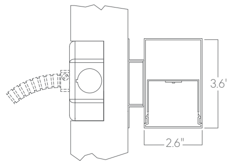
Wall mount
