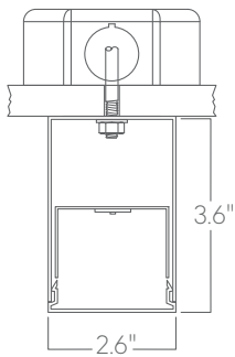
Surface mount
