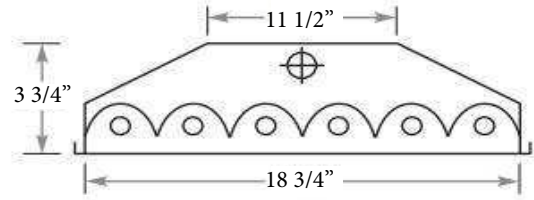
6-LAMP HI-BAY END VIEW
