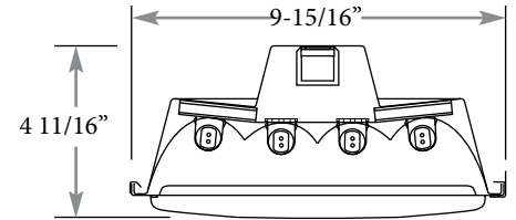
4 LAMP
