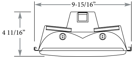
2 LAMP
