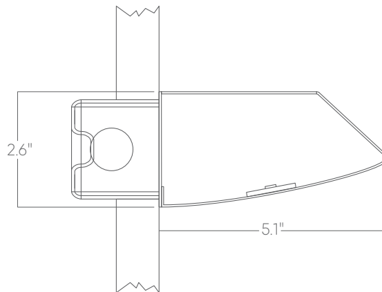
Wall mount
